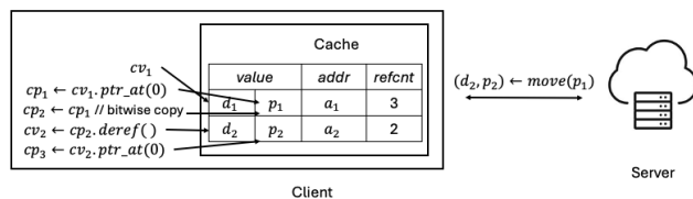
Figure 5: An illustration of how the cache works using a simple client-side program as an example. The client-program uses cache values ( cv_* ) and cache pointers ( cp_* ) to fetch values from the server. Operations performed on cache values and cache pointers are translated into pointer calls that result in legal SAM + programs.
