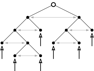
Figure 4: An illustration of our inverted splay tree. Pointers are addresses of leaf nodes of the tree.
